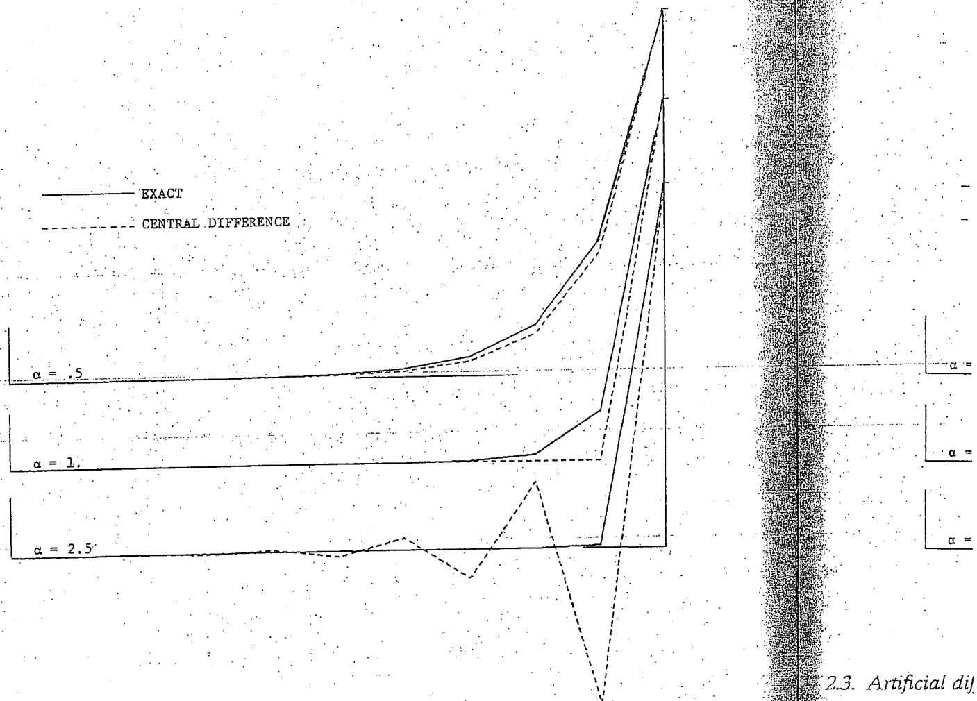
Fig. 2.1. Steady advection-diffusion in one dimension: Central differences.
