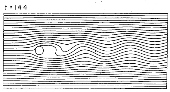
Fig. 6.11. Developing vortex shedding: Streamlines.
