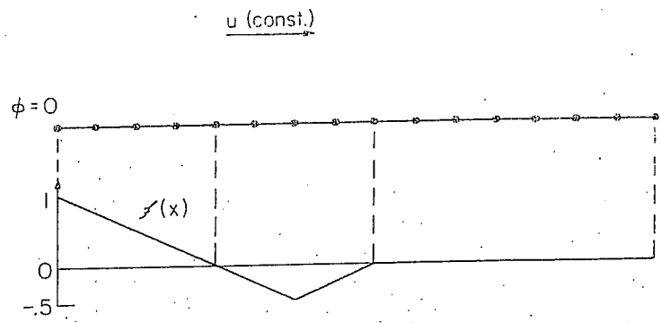
Fig. 3.10. Pure advection with a source term: Problem statement.
