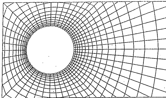
Fig. 6.3. Details of mesh near cylinder.
