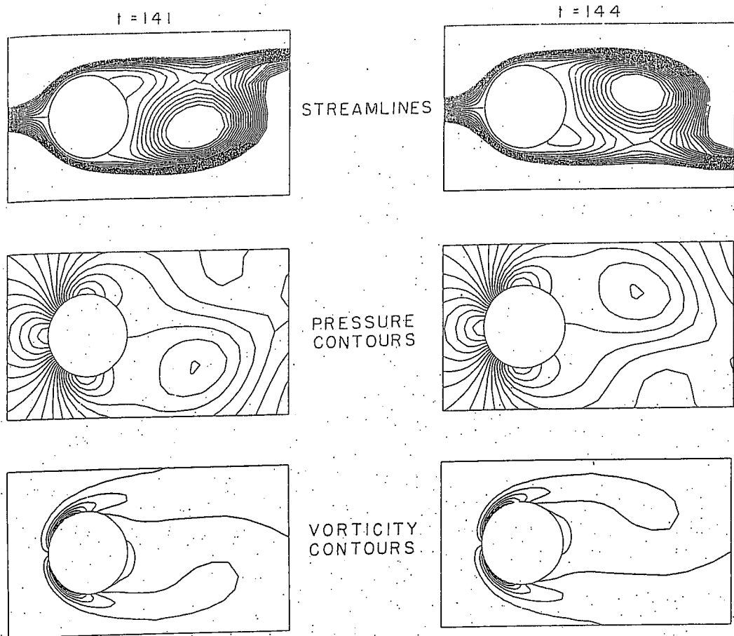
Fig. 6.13. Streamlines, pressure contours and vorticity contours 1/2 cycle apart.
