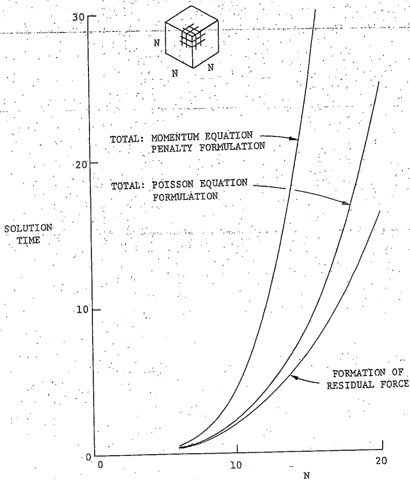
Fig. 5.2. Comparison of solution times: Projected values for three dimensions. (Time is given in CPU seconds per time step per iteration.)
