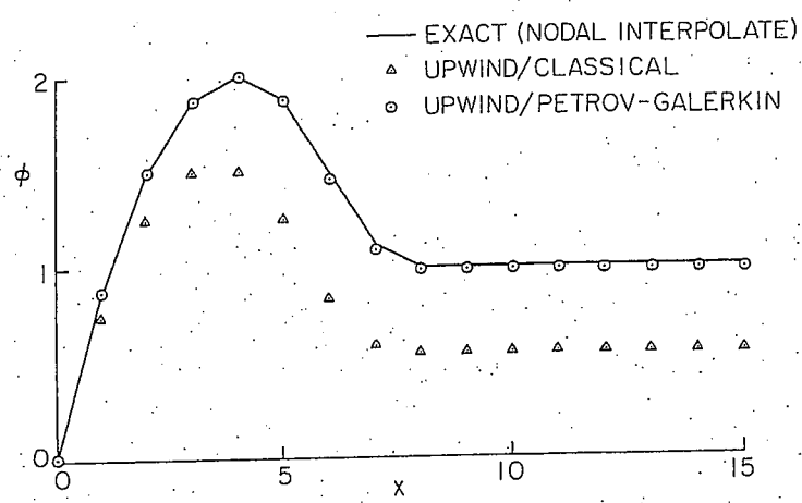
Fig. 3.11. Pure advection with a source term: Comparison of results.
