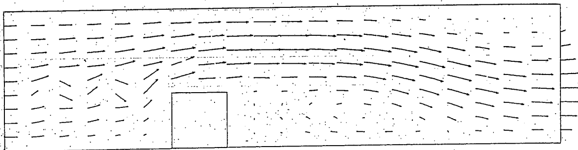
Fig. 1.1. Oscillations generated upstream of a block ( Re = 200 ).
