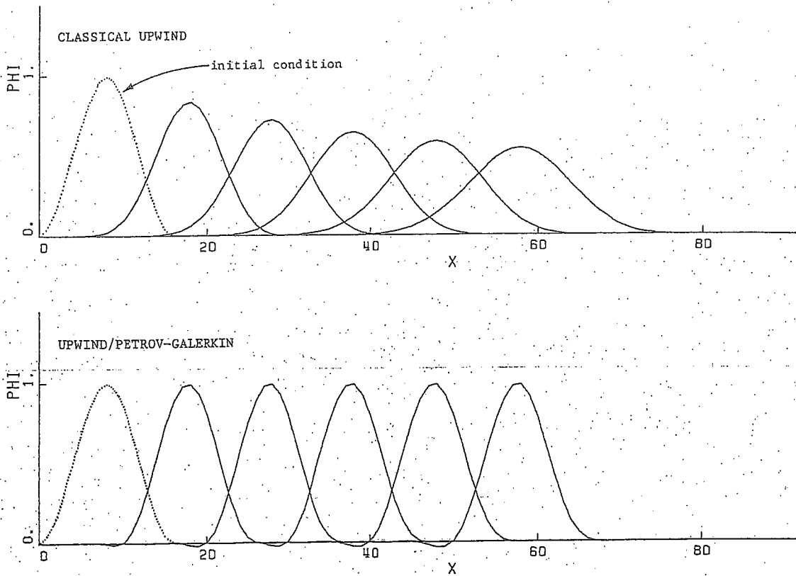
Fig. 3.12. Transient pure advection: Comparison of results at steps 20, 40, 60, 80, and 100.
