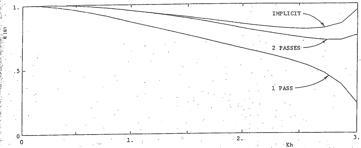
Fig. 4.6. Phase errors for the Petrov-Galerkin transient algorithms.
