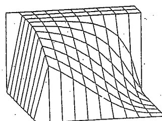
Fig. 3.7. Advection skew to the mesh with homogeneous essential outflow boundary condition: Elevations of \phi .
