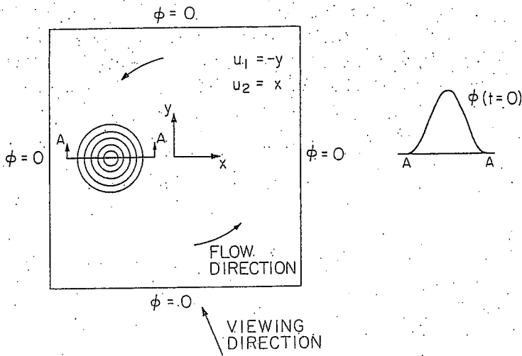
Fig. 3.13. Rotating cone: Problem statement.
