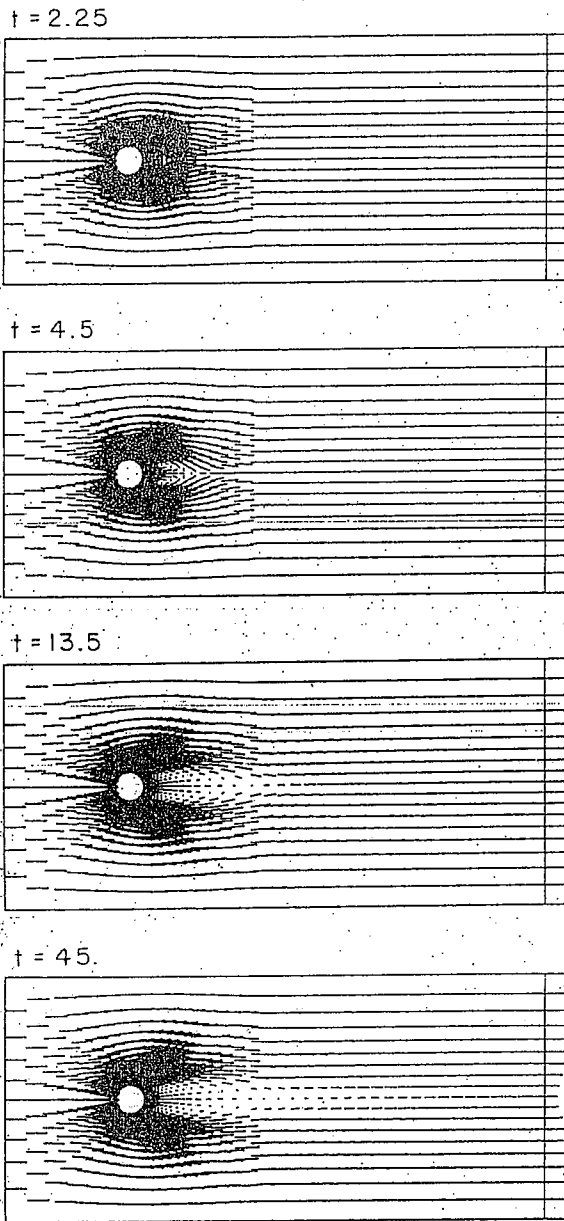
Fig. 6.4. Development of symmetric solution: Velocity vectors.
