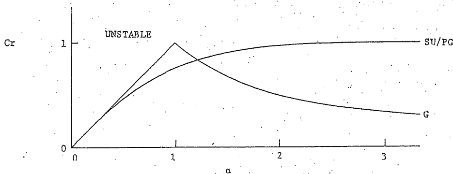
Fig. 4.1. Stability limits for Galerkin (G) and streamline upwind/Petrov-Galerkin (SU/PG) explicit algorithms.
