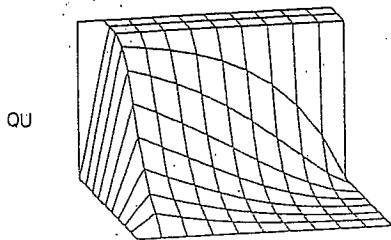
Fig. 3.7. Advection skew to the mesh with homogeneous essential outflow boundary condition: Elevations of \phi .
