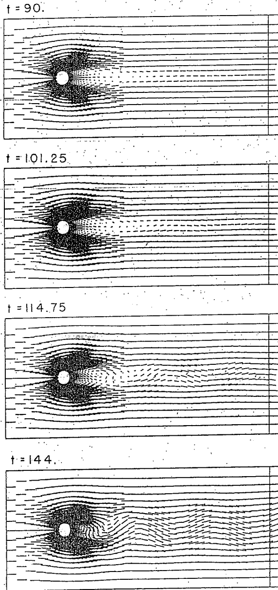
Fig. 6.10. Developing vortex shedding: Velocity vectors.
