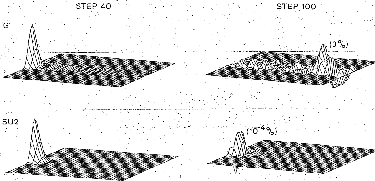
Fig. 3.15. Cone impinging on a natural-boundary-condition boundary. Amplitude of residual values, as a percentage of initial cone height, shown in parentheses.
