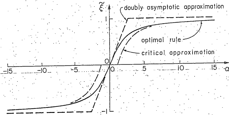
Fig. 3.3. Integration rule for optimal upwind scheme, doubly asymptotic approximation, and critical approximation.
