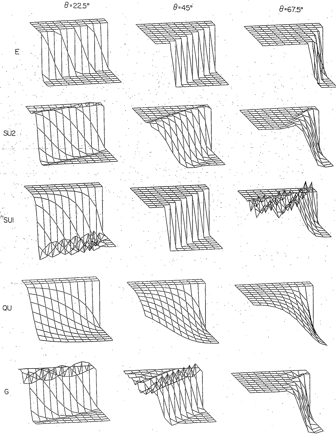
Fig. 3.6. Advection skew to the mesh with homogeneous natural outflow boundary condition: Elevations of \phi .
