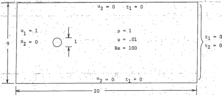
Fig. 6.1. Flow past a cylinder: Problem statement.
