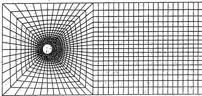
Fig. 6.2. Finite element mesh; 1510 nodes, 1436 elements.
