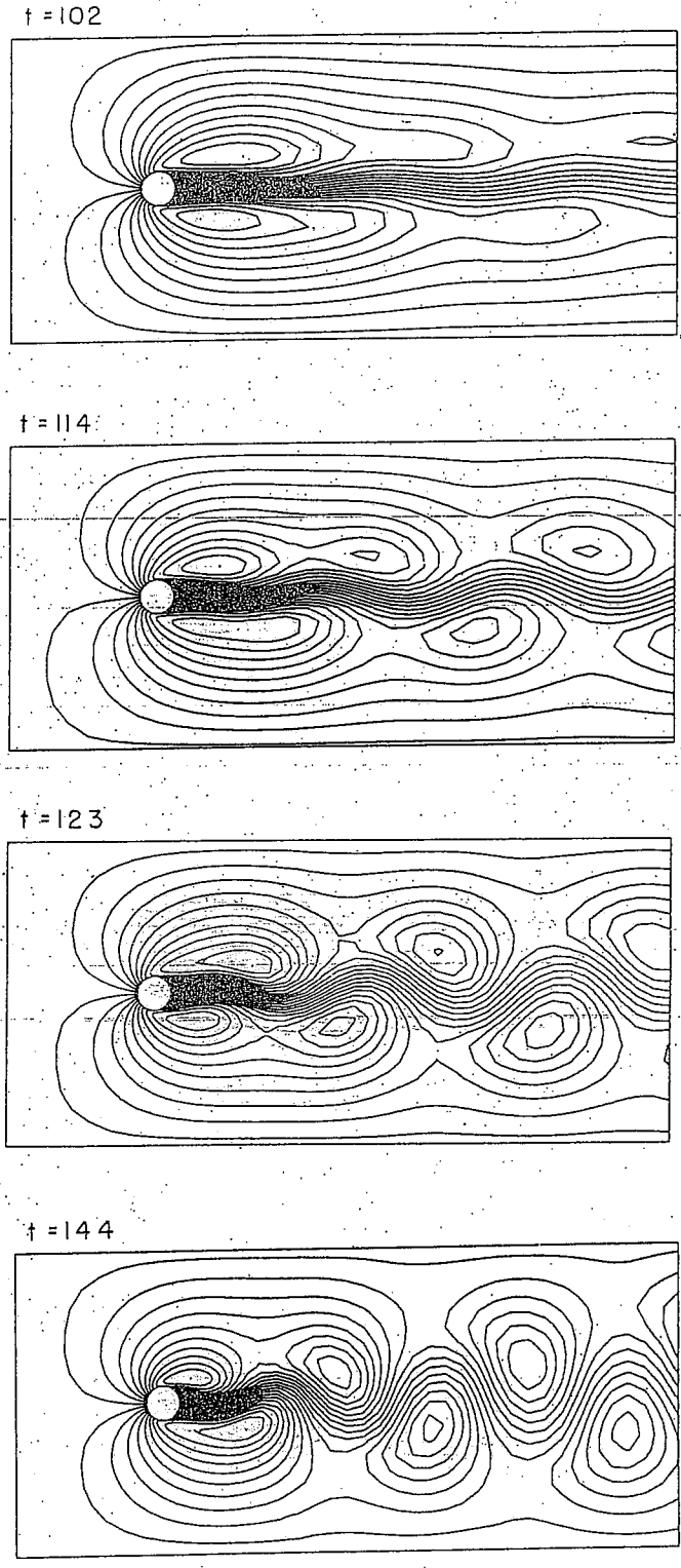
Fig. 6.12. Developing vortex shedding: Stationary streamlines.
