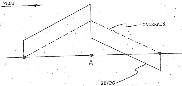
Fig. 3.2. Comparison of streamline upwind/Petrov-Galerkin (SU/PG) and Galerkin weighting functions for node A.
