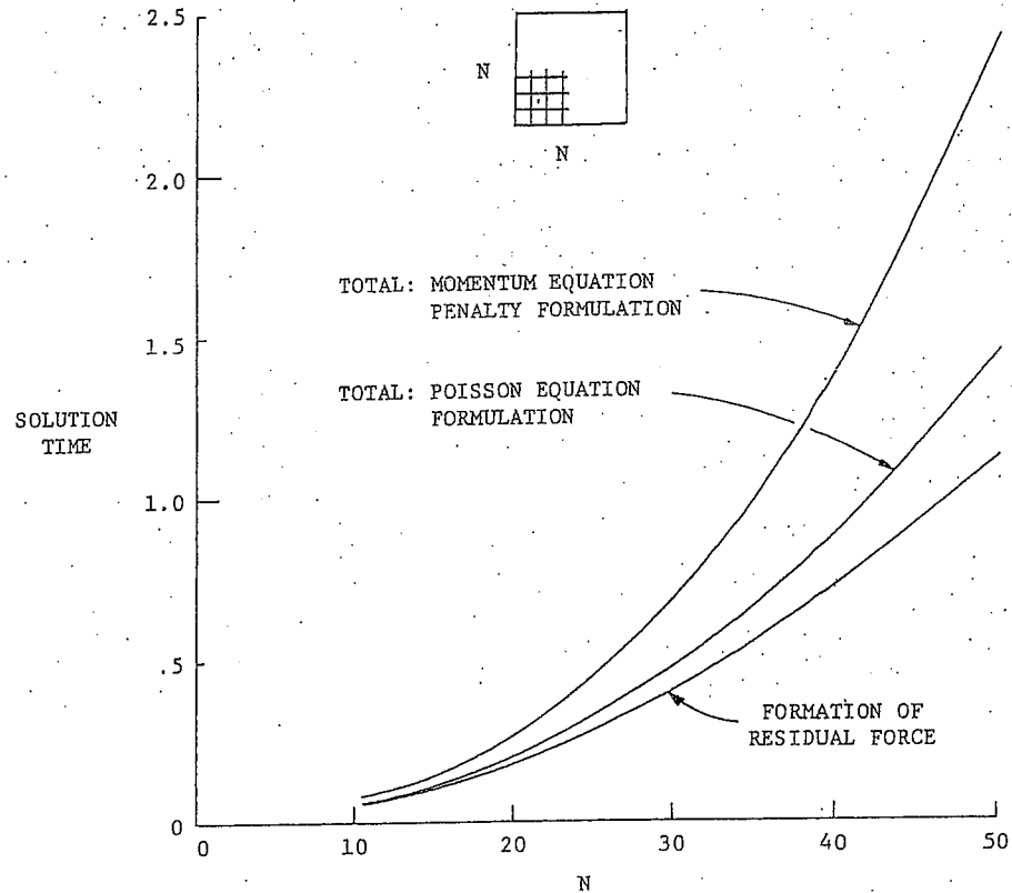
Fig. 5.1. Comparison of solution times: Two dimensions. (Time is given in CPU seconds per time step per iteration.) The difference between the total and the formation of the residual force represents the time for equation solving.
