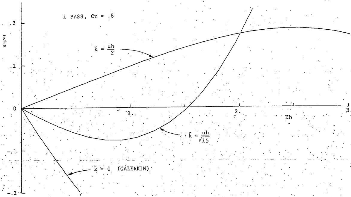
Fig. 4.2. Effect of Petrov-Galerkin parameter, \bar{k} , on algorithmic damping ratio: Pure advection, one pass (Negative values result in instability.)
