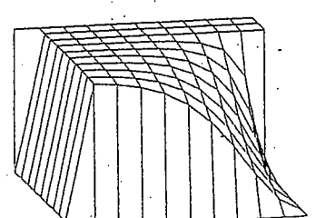
Fig. 3.7. Advection skew to the mesh with homogeneous essential outflow boundary condition: Elevations of \phi .
