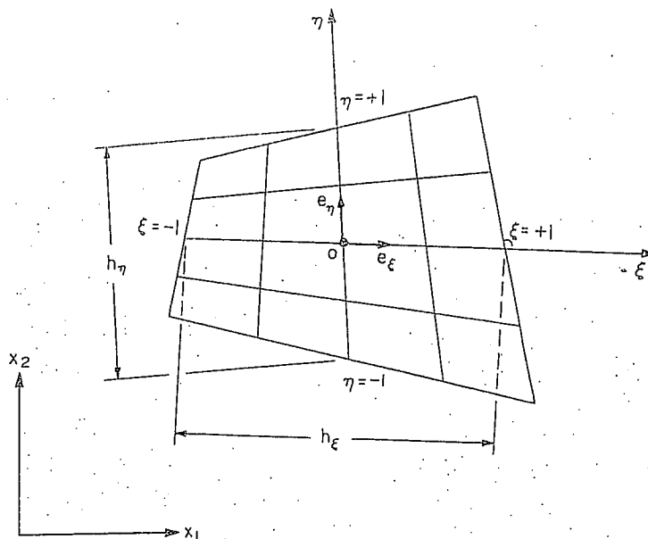
Fig. 3.4. Typical four-node quadrilateral finite element geometry.
