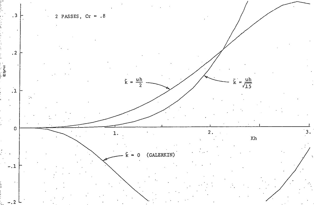
Fig. 4.3. Effect of Petrov-Galerkin parameter, \bar{k} , on algorithmic damping ratio; Pure advection, two passes. (Negative values result in instability.)
