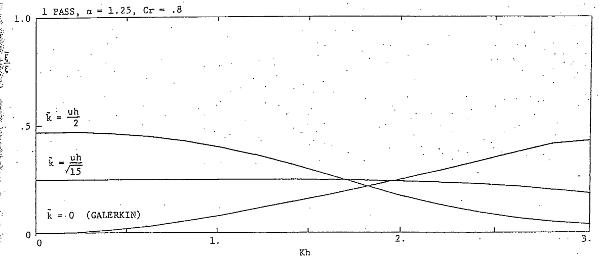
Fig. 4.4. Ratio of numerical damping, \bar{\xi} , to physical damping, \xi , for different values of Petrov-Galerkin parameter, \bar{k} : One pass.
