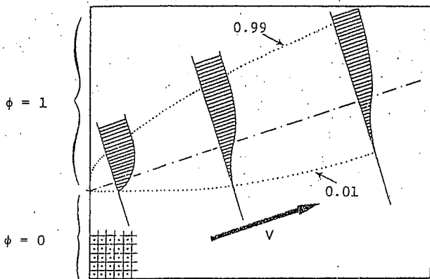
Fig. 3.1. Illustration of the crosswind diffusion problem: \alpha = 100 (from ref. [33]).
