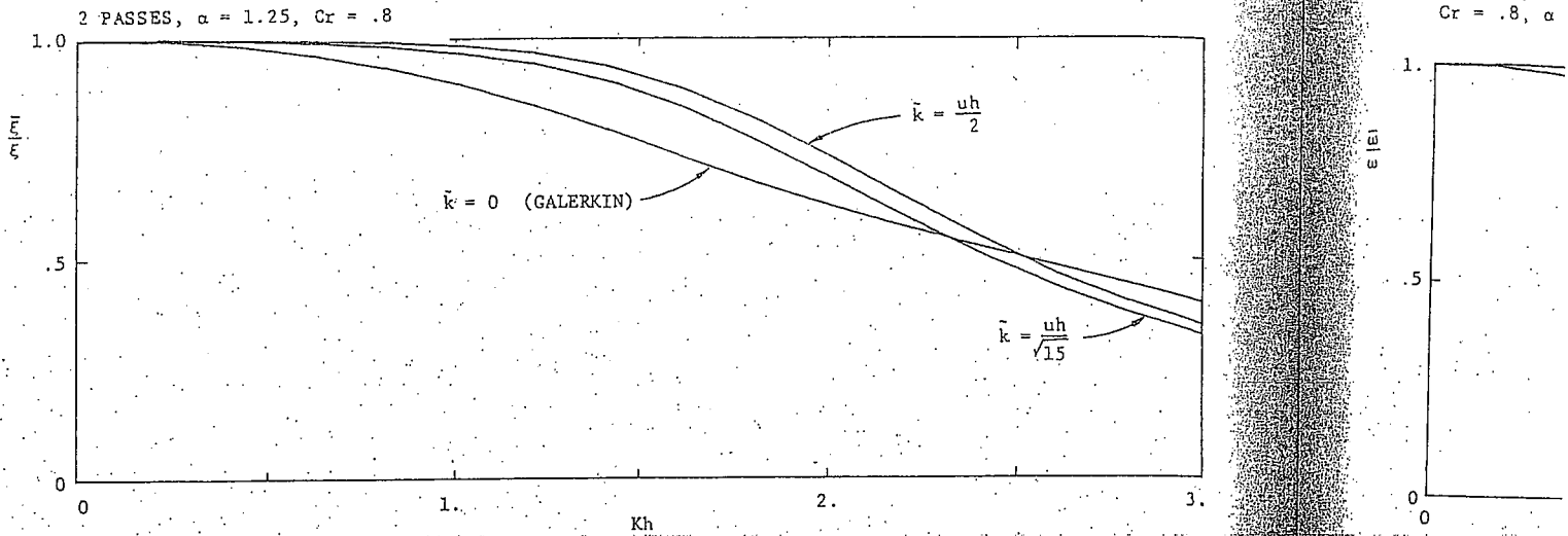
Fig. 4.5: Ratio of numerical damping, \bar{\xi} , to physical damping, \xi , for different values of Petrov-Galerkin parameter, \bar{k} : Two passes.
