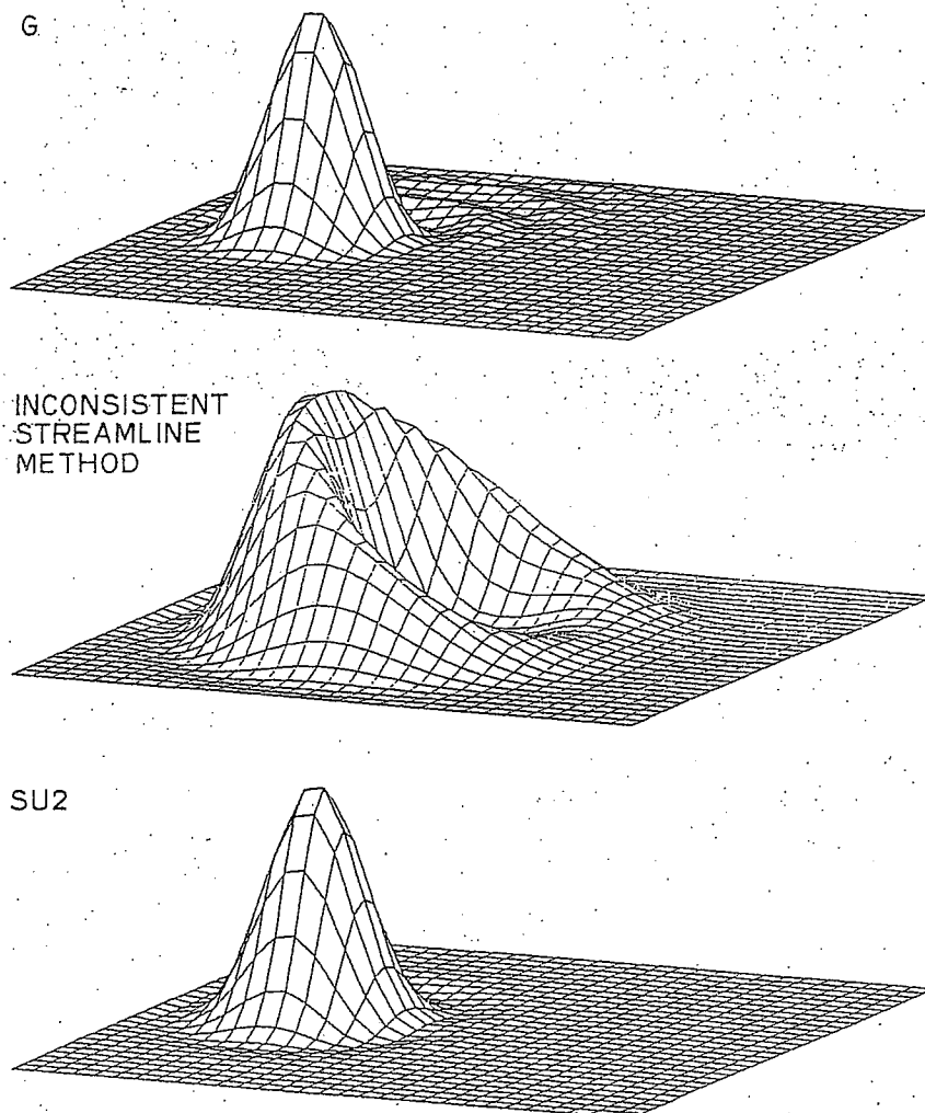
Fig. 3.14. Rotating cone: Elevations of \phi after one rotation (200 time steps).
