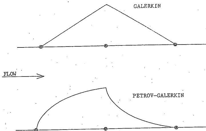
Fig. 2.3. Galerkin weighting function and upwind Petrov-Galerkin weighting function.
