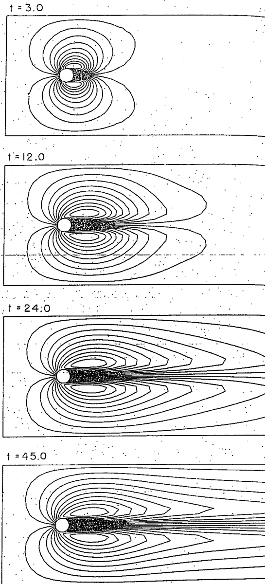
Fig. 6.5. Development of symmetric solution: Stationary streamlines.
