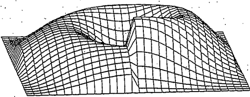
Fig. 3.9. Advection in a rotating flow field: Elevations of \phi .
